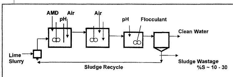
Figure 3. High Density Sludge "HDS" Process.
