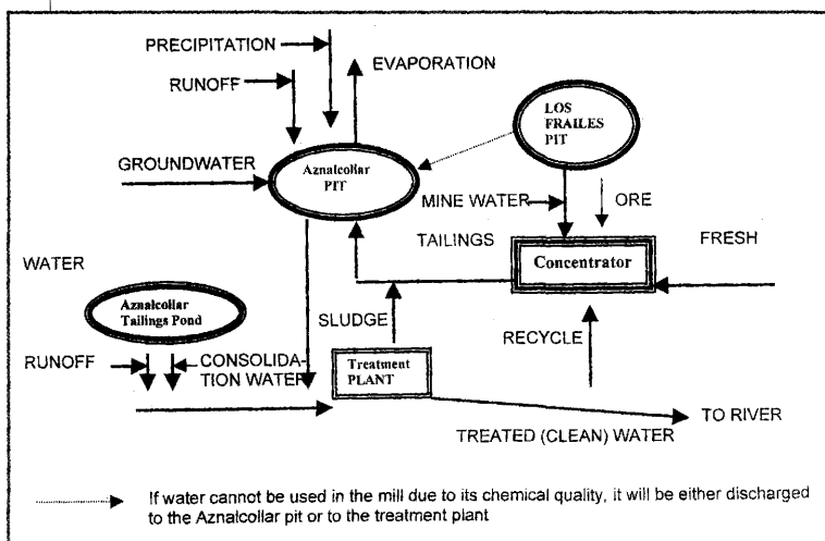
Figure 1. Water Management at the Boliden Apirsa Site.
