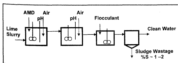
Figure 2. Lime addition to neutralization reactors: Basic-Conventional Method.
