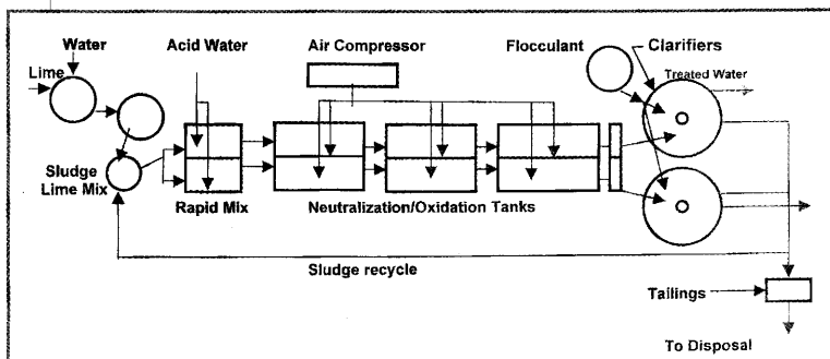
Figure 4. Boliden Apirsa HDS lime neutralization treatment plant.
